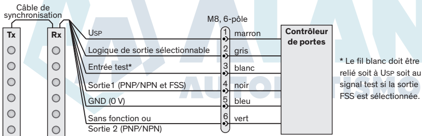
Figure 10: Schéma de raccordement
